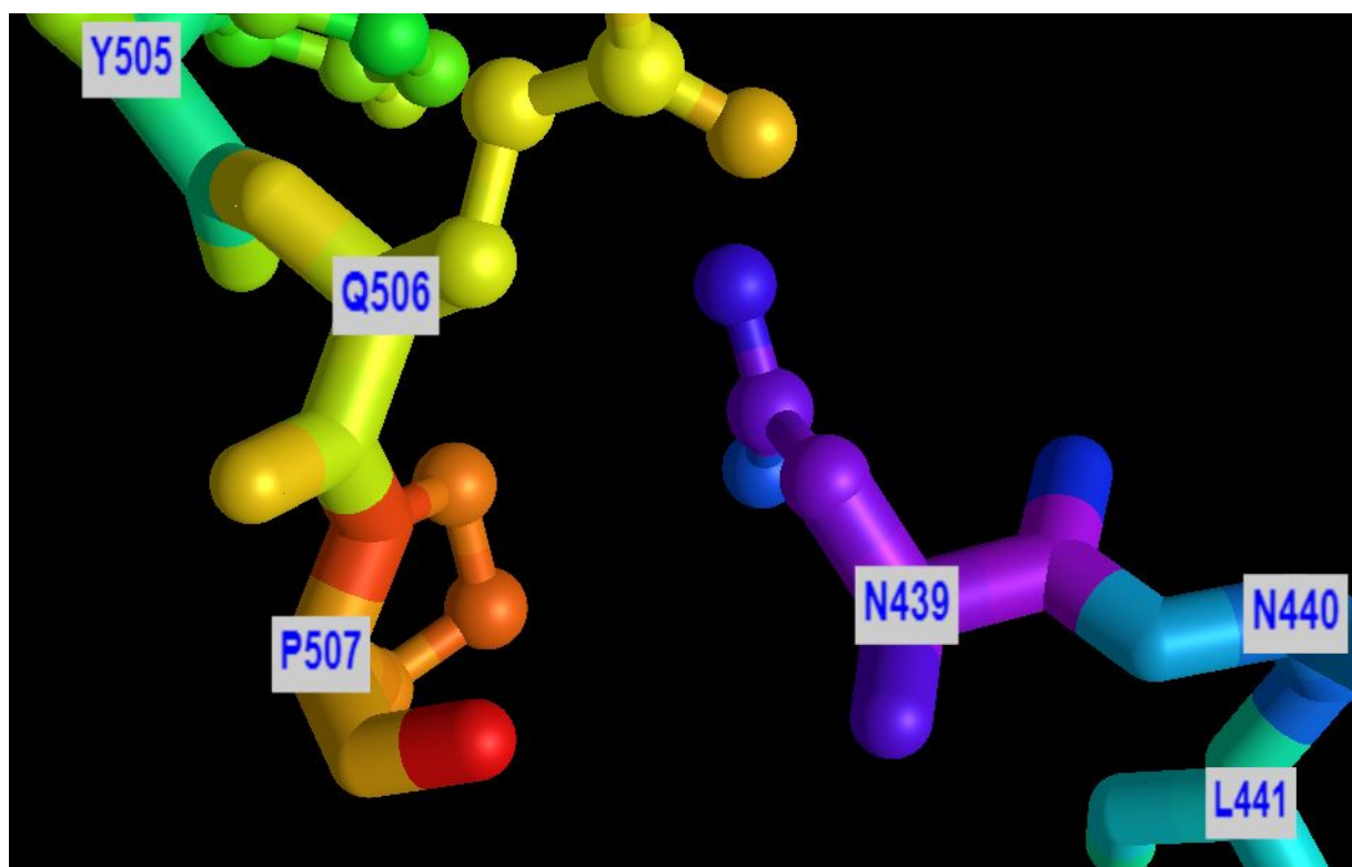
Figure: Linker portion of the peptide Spike N501Y-s, shown in the context of the wild-type Spike protein (PDB ID 6XM4). In the peptide Spike N501Y-s, the C-terminus of Pro507 (shown here in
